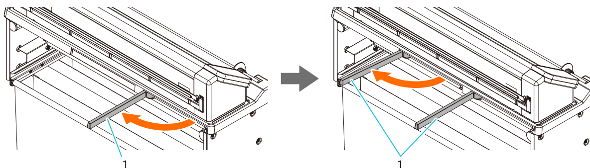
1. Support bar
